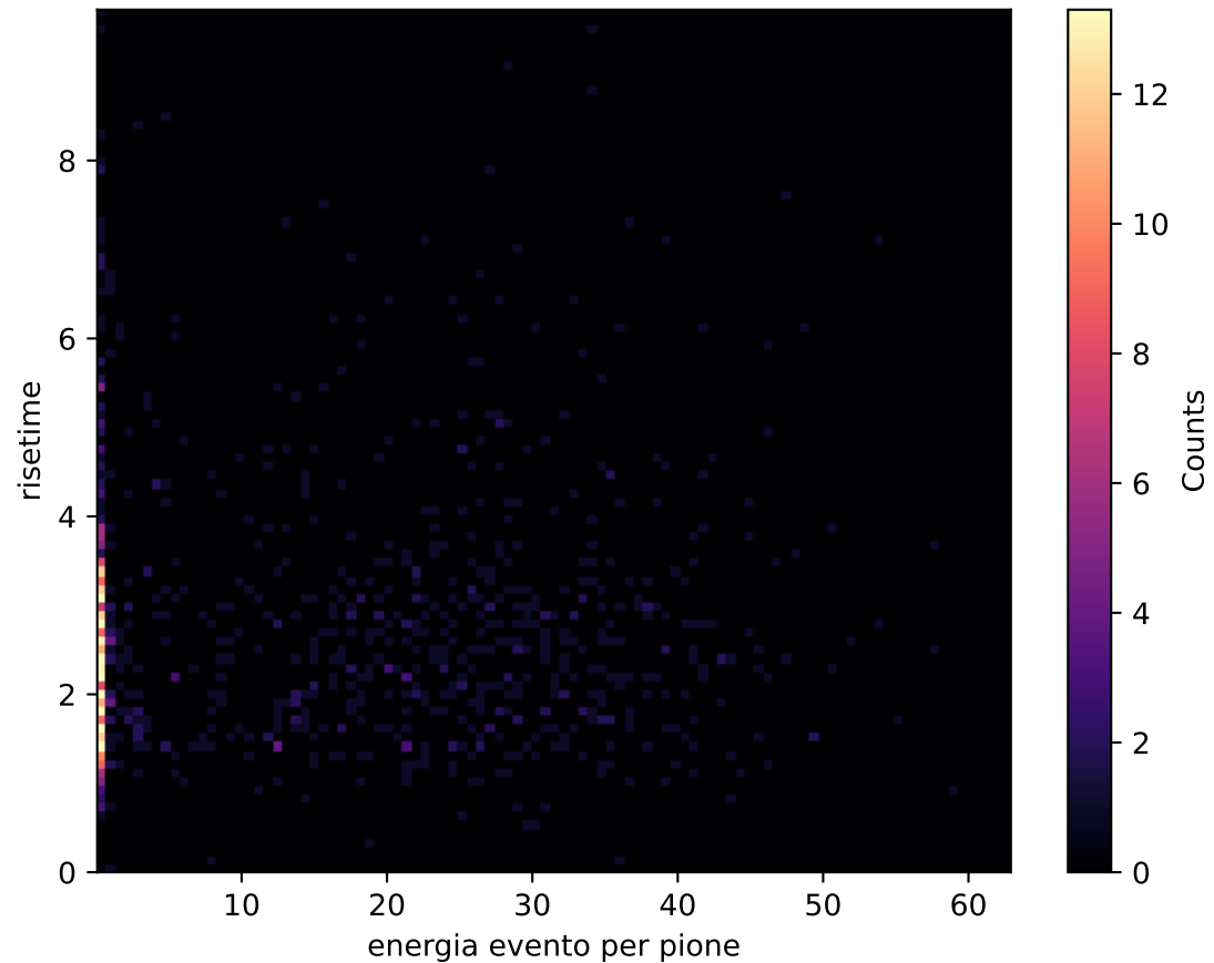
pion distribution 60.0GeV
