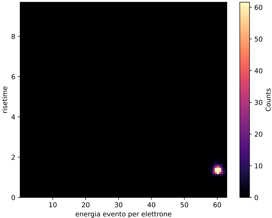
electron distribution 60.0GeV
